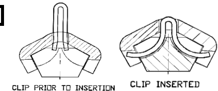
Cast Wedge & Retaining clip
